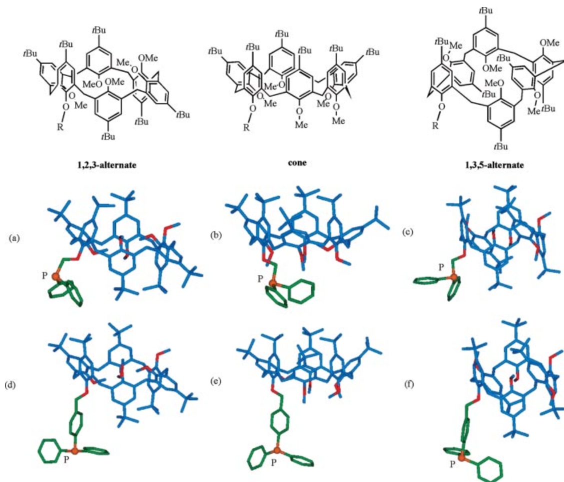
Figure 3. Conformers and optimized structures (B3LYP/LANL2DZ–CONFLEX5/MMFF94s) of 3 [(a) 1,2,3-alternate, (b) cone, (c) 1,3,5-alternate] and 5 [(d) 1,2,3-alternate, (e) cone, (f) 1,3,5-alternate].
