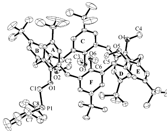
Figure 1. ORTEP drawing of the molecular structure of 3 with thermal ellipsoids at 50% probability levels. Hydrogen atoms have been omitted for clarity.
