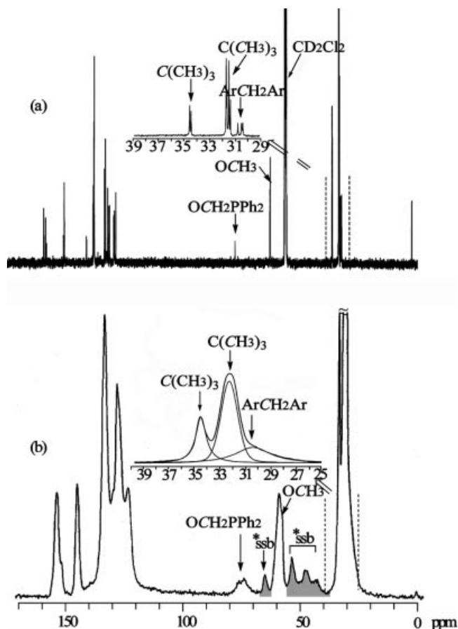
Figure 2. ^{13}\text{C}\{^1\text{H}\} NMR spectra of 3 at 25 °C: (a) measured in \text{CD}_2\text{Cl}_2 ; (b) measured in the solid state (CPMAS). *ssb: spinning side-band.
