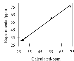
Figure 4. Correlation plots of the calculated vs. experimental ^{13}\text{C} NMR chemical shifts for the cone conformer.
