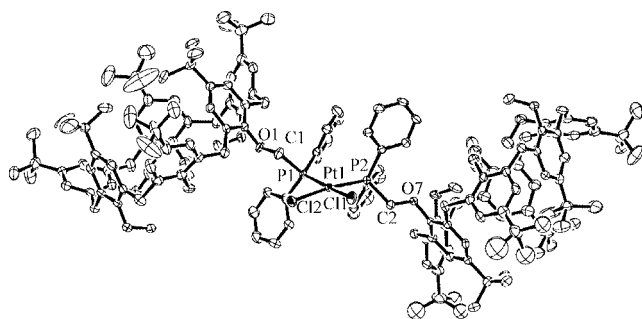
Figure 5. ORTEP drawing of [\text{PtCl}_2(\mathbf{3})_2] with thermal ellipsoids at 50% probability levels. Hydrogen atoms have been omitted for clarity.
